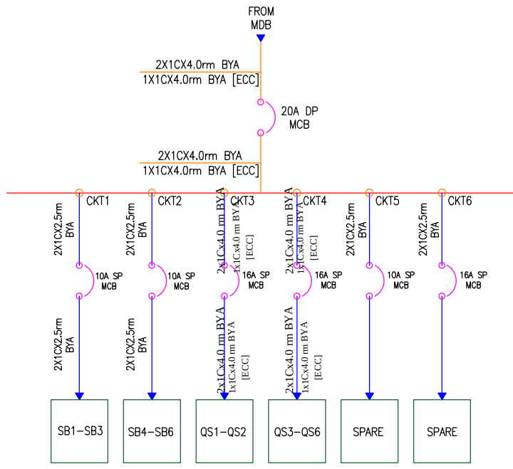
SDB-1 SINGLE LINE DIAGRAM
