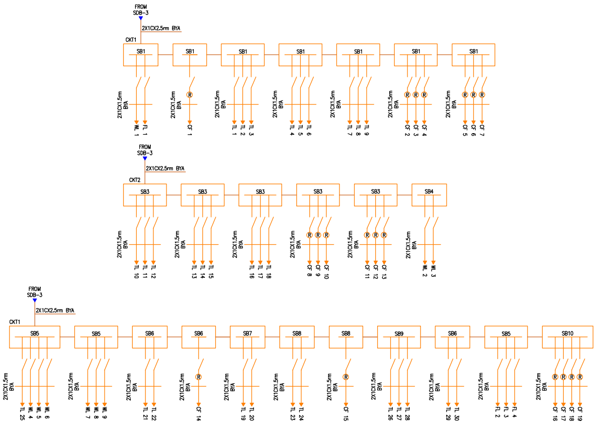
SDB-3 CIRCUIT DIAGRAM
