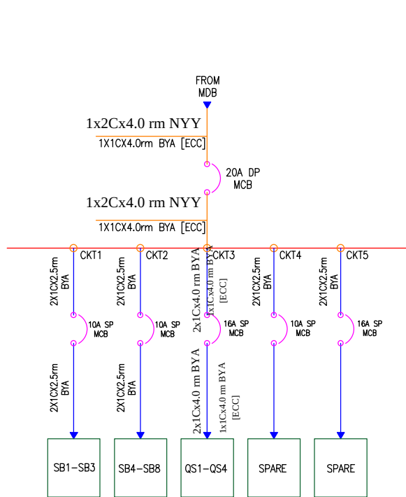
SDB-2 SINGLE LINE DIAGRAM
