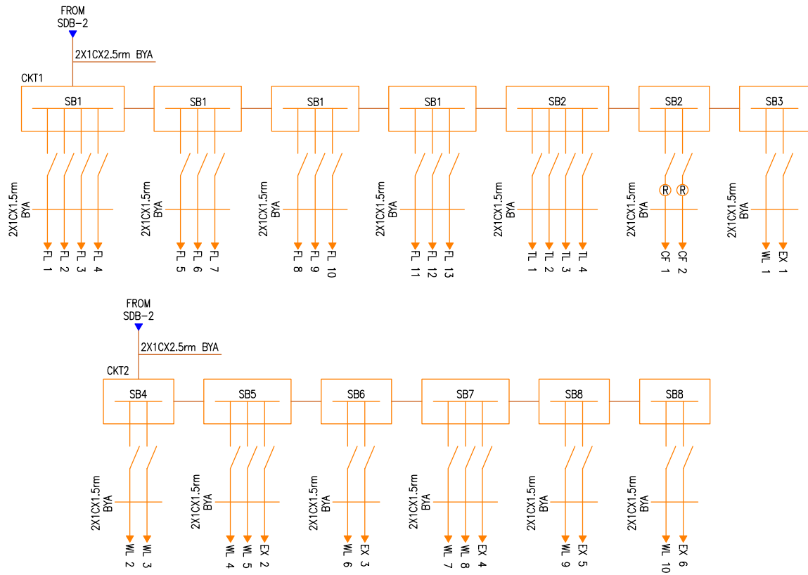
SDB-2 CIRCUIT DIAGRAM
