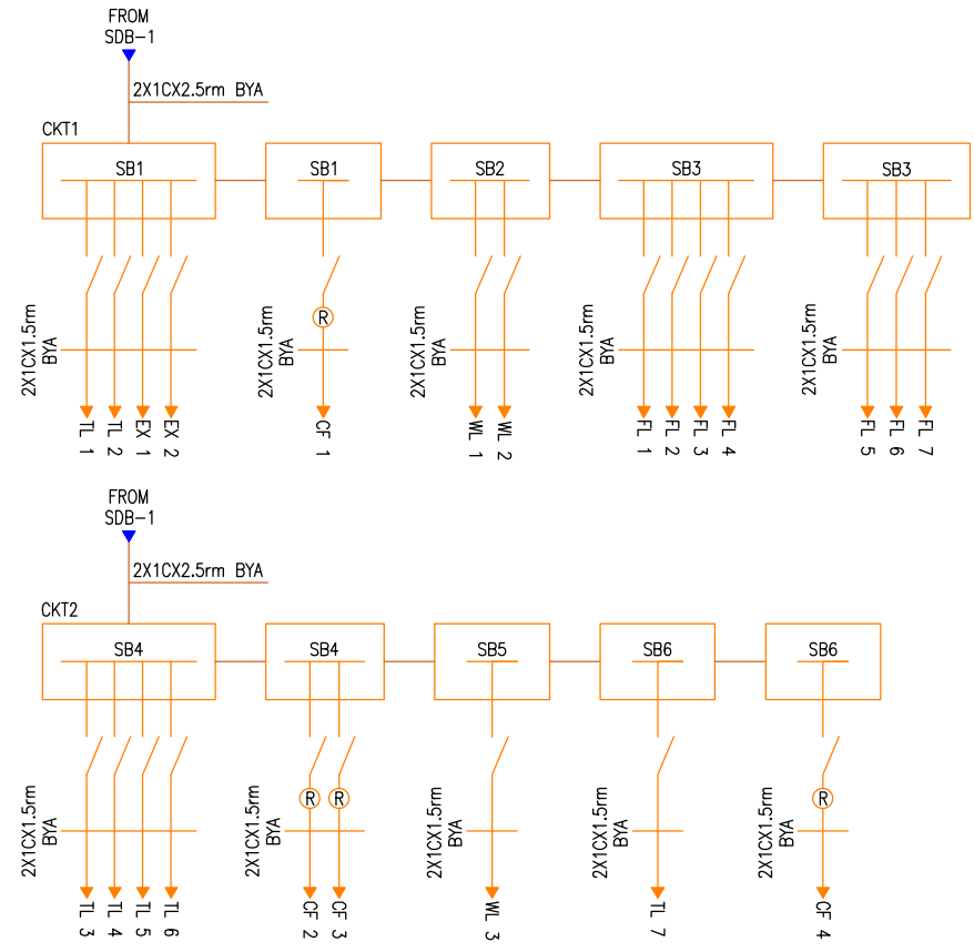
SDB-1 CIRCUIT DIAGRAM
