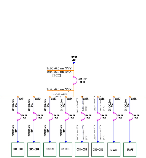
SDB-3 SINGLE LINE DIAGRAM
