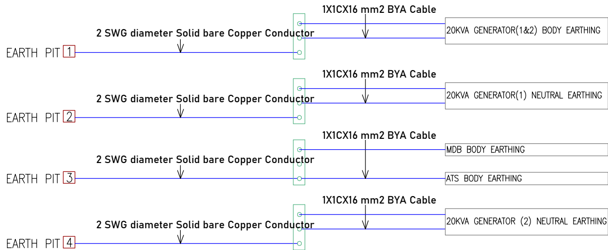
Earthing Layout Drawing
