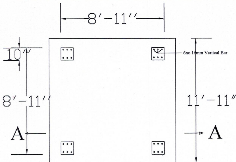
Plan of Colum
