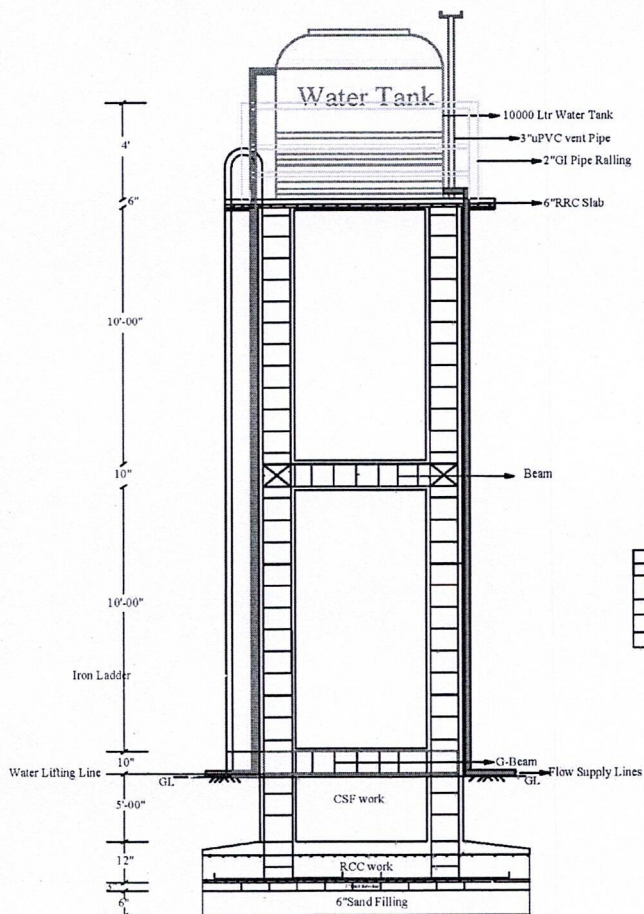
X-Section of Footing and colum
