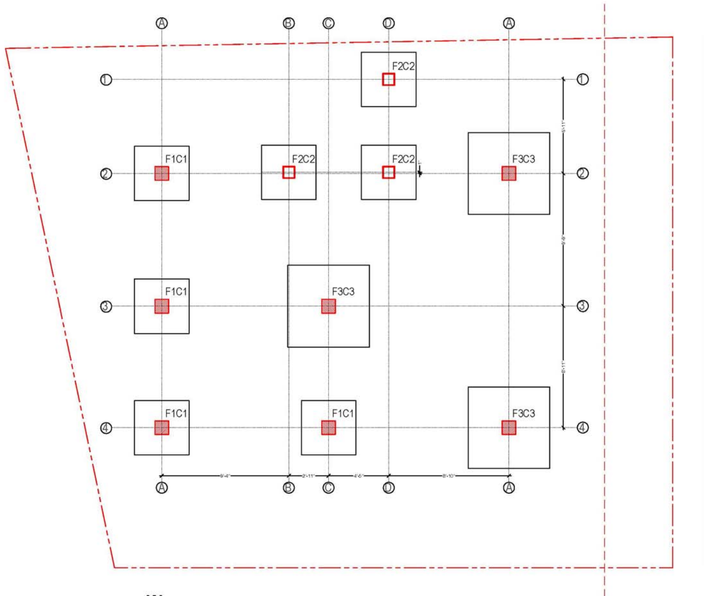
W N Foundation Layout Plan
