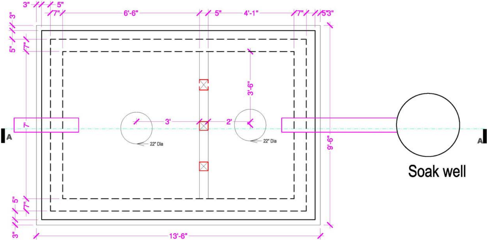
SEPTIC TANK DETAILS
