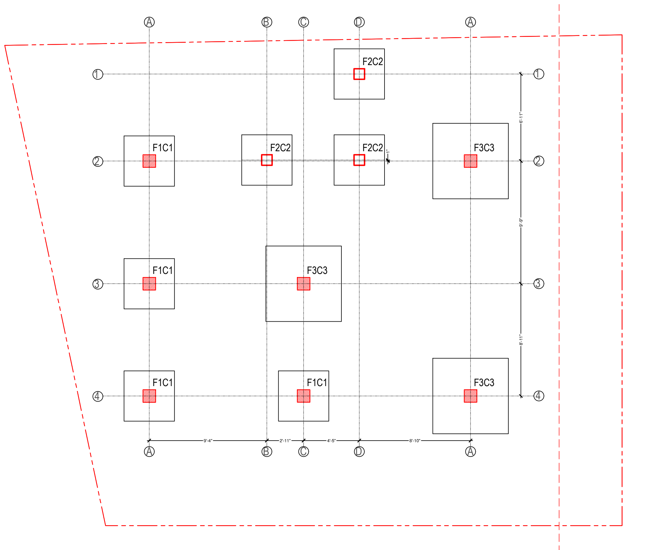
W N Foundation Layout Plan
