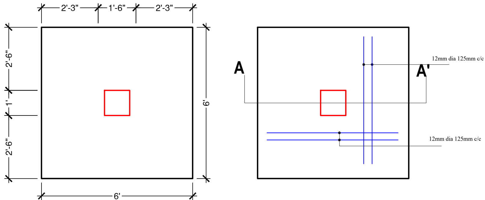
F3C3 PLAN
